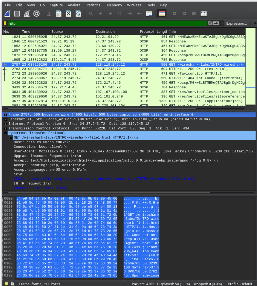
Figure 5: Wireshark window after step 9
