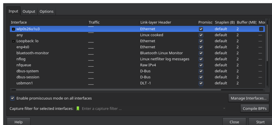
Figure 4: Wireshark Capture Interface Window
