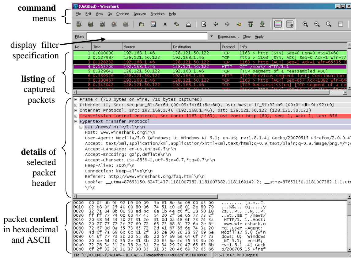
Figure 3: Wireshark GUI during packet capture and analysis
