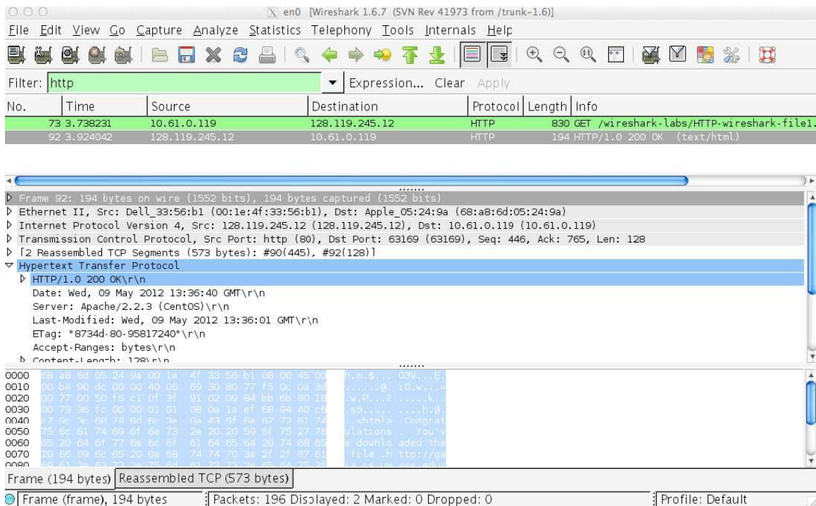
Figure 1: Wireshark Display After Retrieving the Webpage
